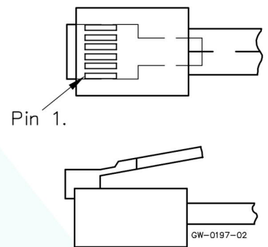
Modular cable with connector.
