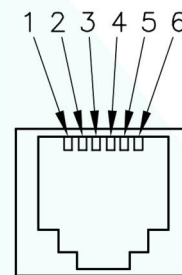
Modular jack
